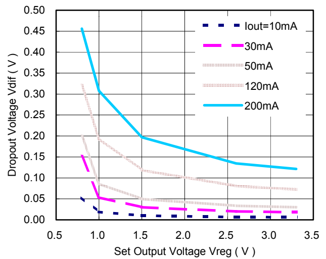
R1160NXX1X ECO=L
