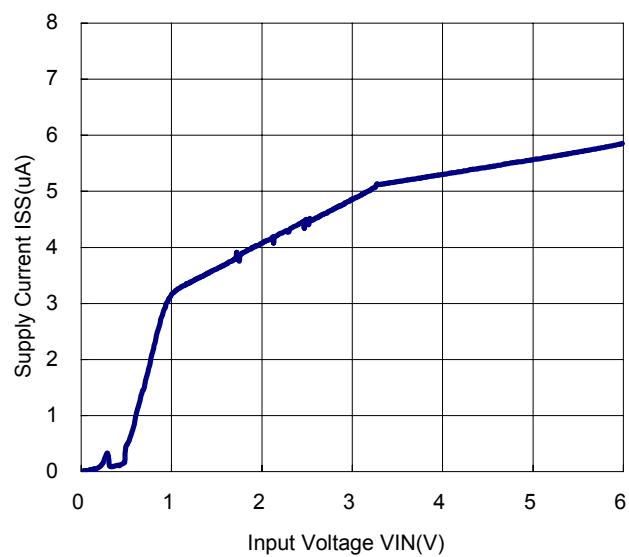
R1160N331X ECO=L
