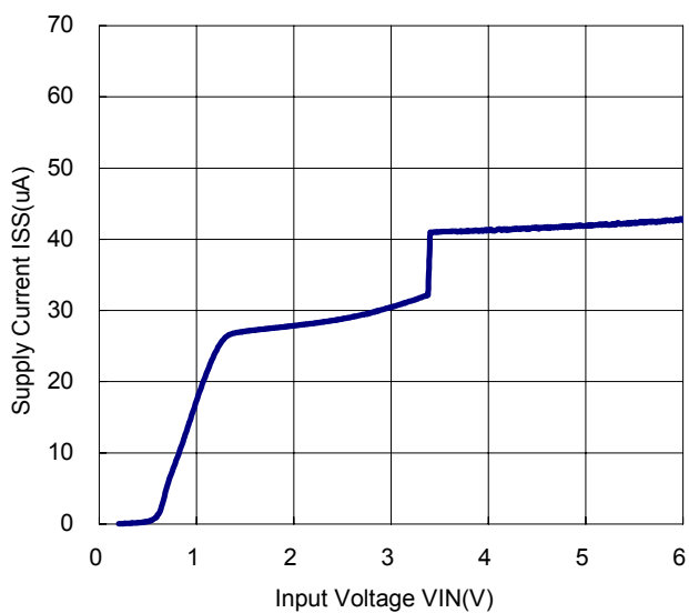
R1160N331X ECO=H
