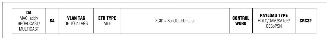
Figure 1-9. TDMoMEF Packet with VLAN Tag
