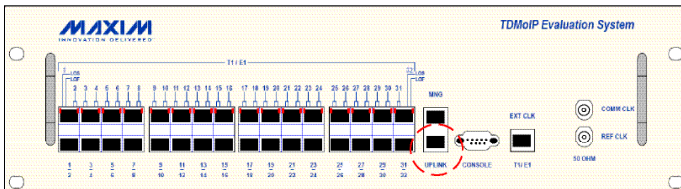
Figure 2-3. UPLINK Connector
