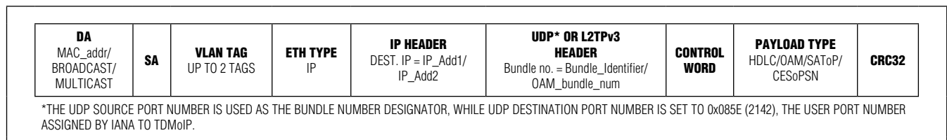
Figure 1-7. TDMoIP Packet with VLAN Tag
