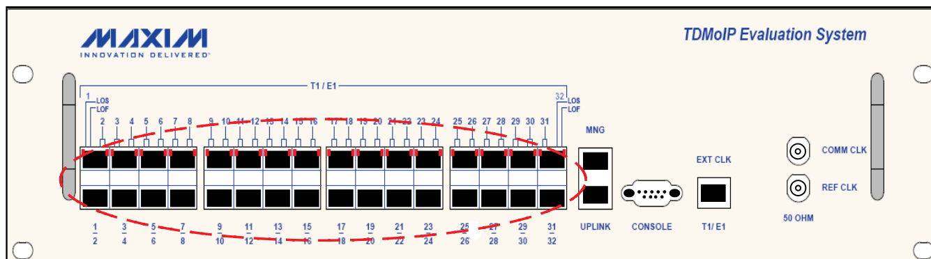
Figure 2-4. T1/E1 Connectors
