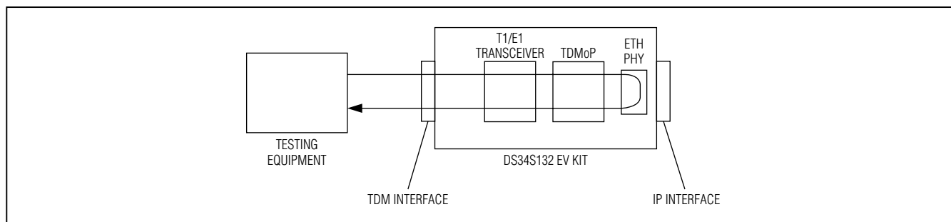
Figure 5-13. PHY Loopback Diagram
