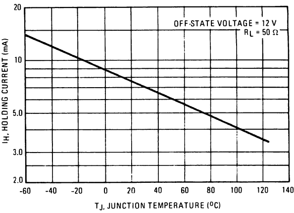
FIGURE 9 – HOLDING CURRENT
