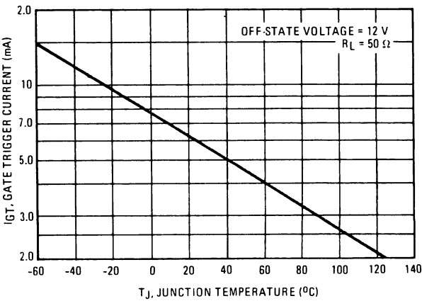
FIGURE 7 – GATE TRIGGER CURRENT
