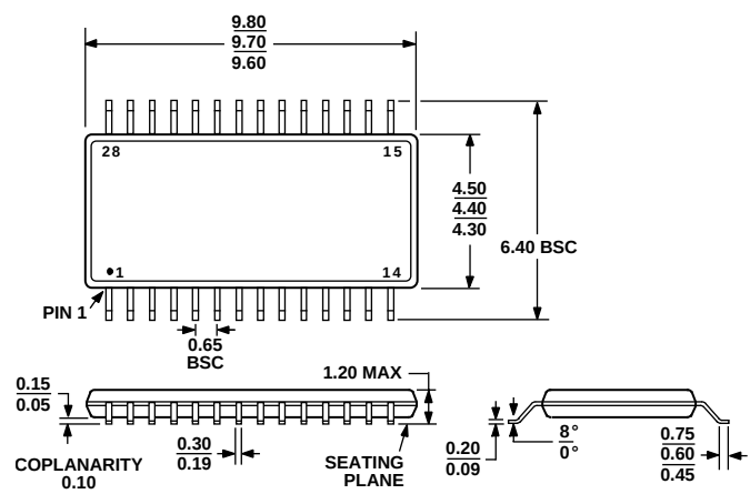
COMPLIANT TO JEDEC STANDARDS MO-153-AE Figure 45. 28-Lead Thin Shrink Small Outline Package [TSSOP] (RU-28) Dimensions shown in millimeters
