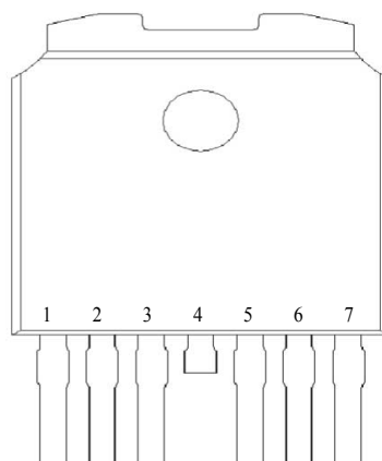
Figure 2. Configuration diagram (top view)
