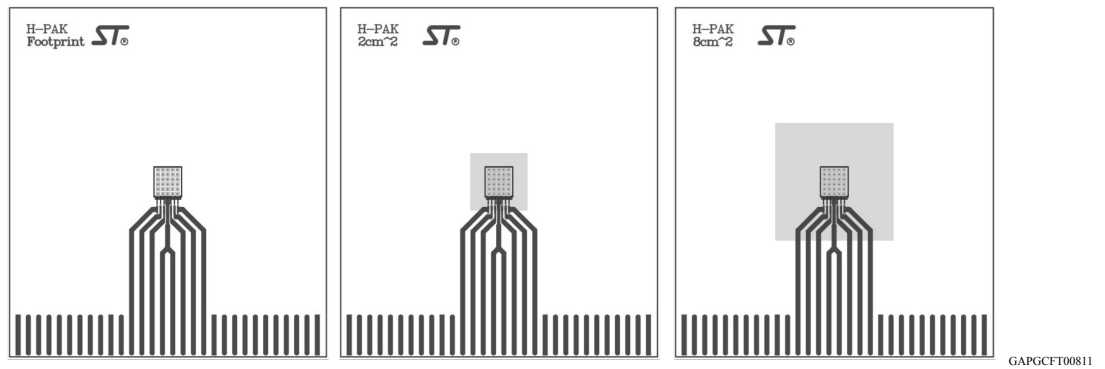
Figure 26. HPAK PCB
