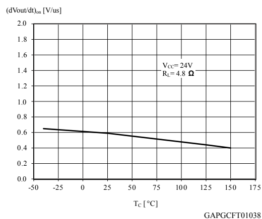
Figure 22. Turn-on voltage slope
