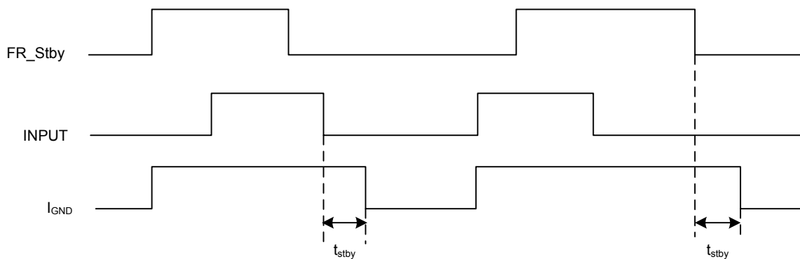
Figure 5. t_{\text{stby}} definition
