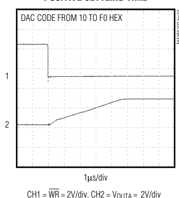
POSITIVE SETTLING TIME
