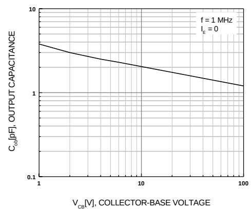
Figure 6. Output Capacitance
