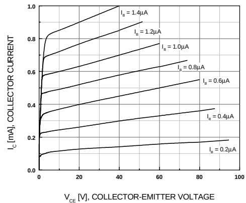
Figure 2. Static Characteristics
