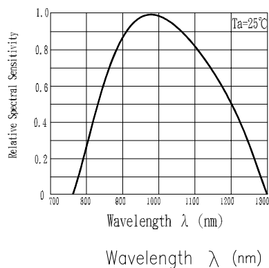
Fig.5 Spectral Sensitivity
