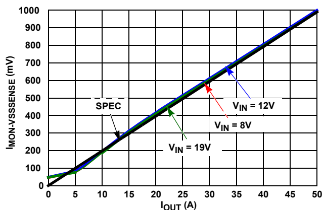
FIGURE 52. IMON, V_{ID} = 1.075
