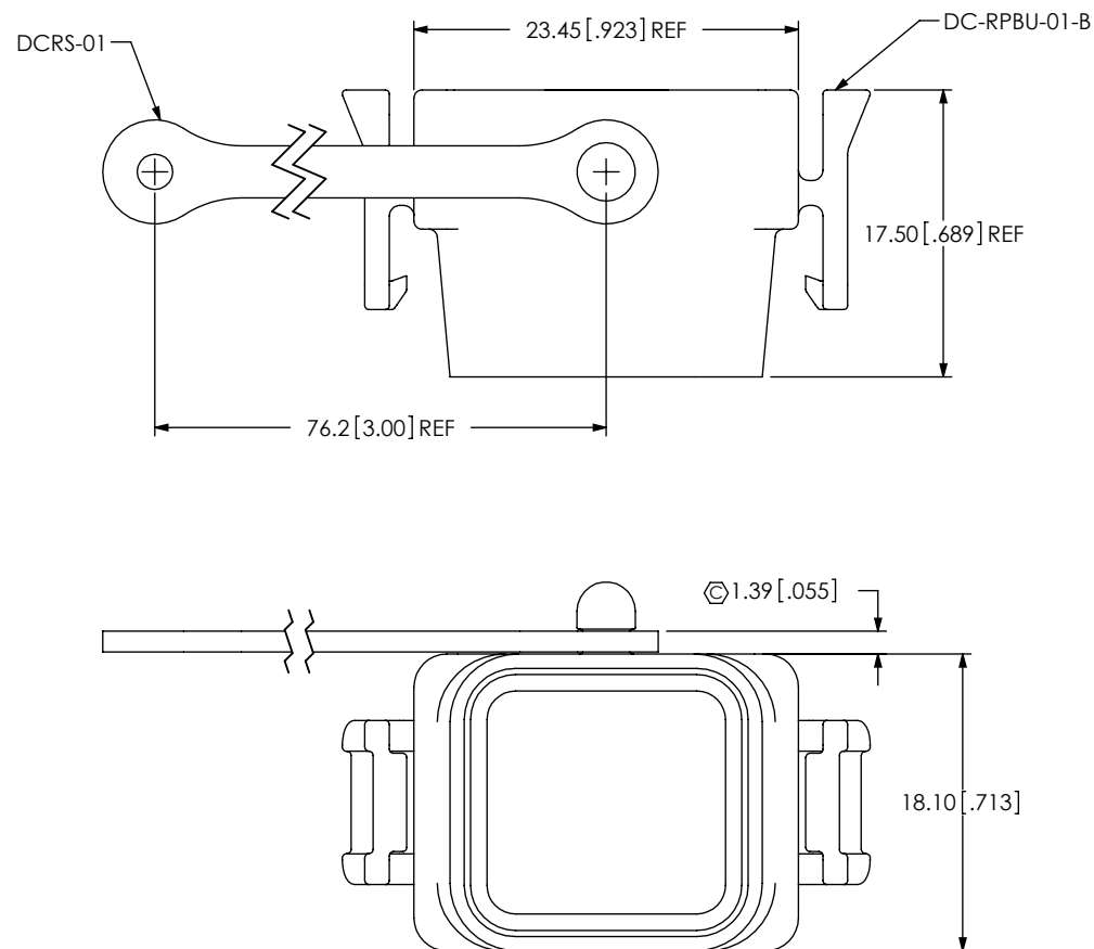
FIG. 2 DCA-RPBU-01-01-B SHOWN (FOR RPBU-01-X-B-XX-XX PANEL ONLY)
