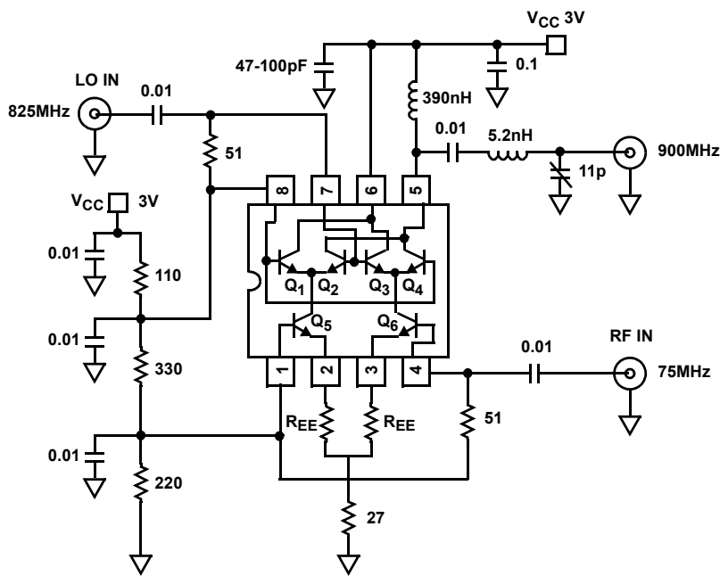
FIGURE 12. UP CONVERTER
