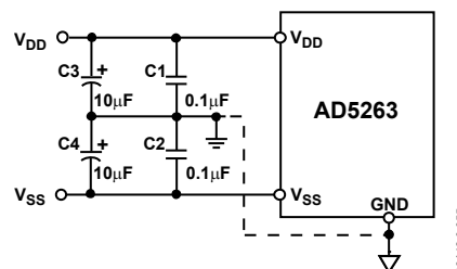
Figure 54. Power Supply Bypassing
