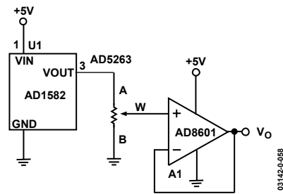
Figure 58. Programmable Voltage Reference
