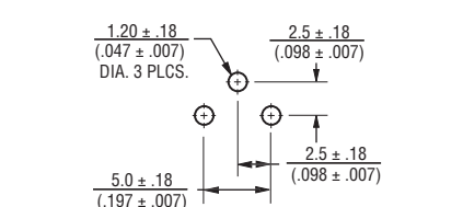
SUGGESTED PWB LAYOUT
