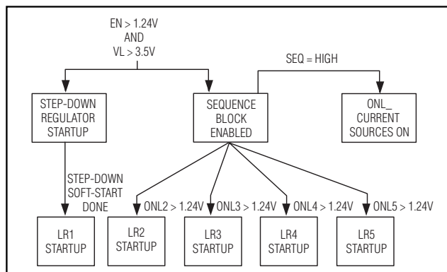
Figure 5. Startup Conditions
