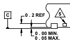
DETAIL "X"
