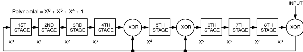
1-WIRE CRC GENERATOR Figure 4
