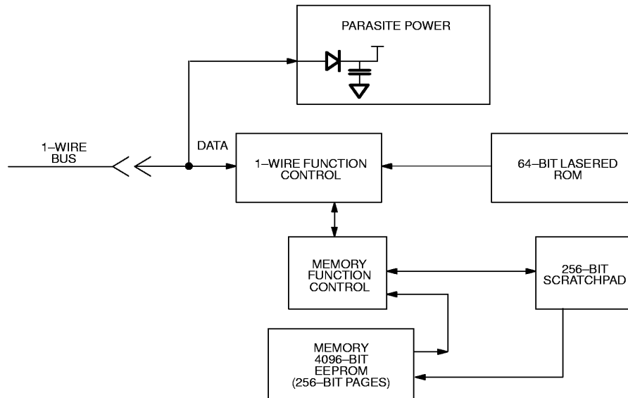
DS2433 BLOCK DIAGRAM Figure 1
