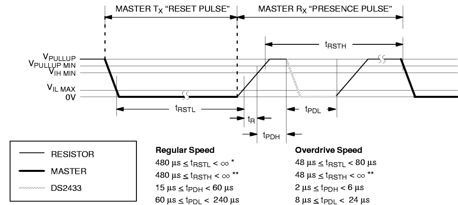
INITIALIZATION PROCEDURE RESET AND PRESENCE PULSES Figure 10
