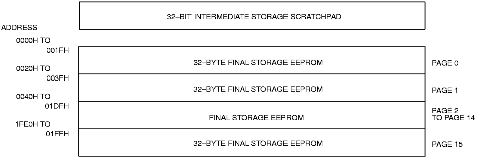
DS2433 MEMORY MAP Figure 5
