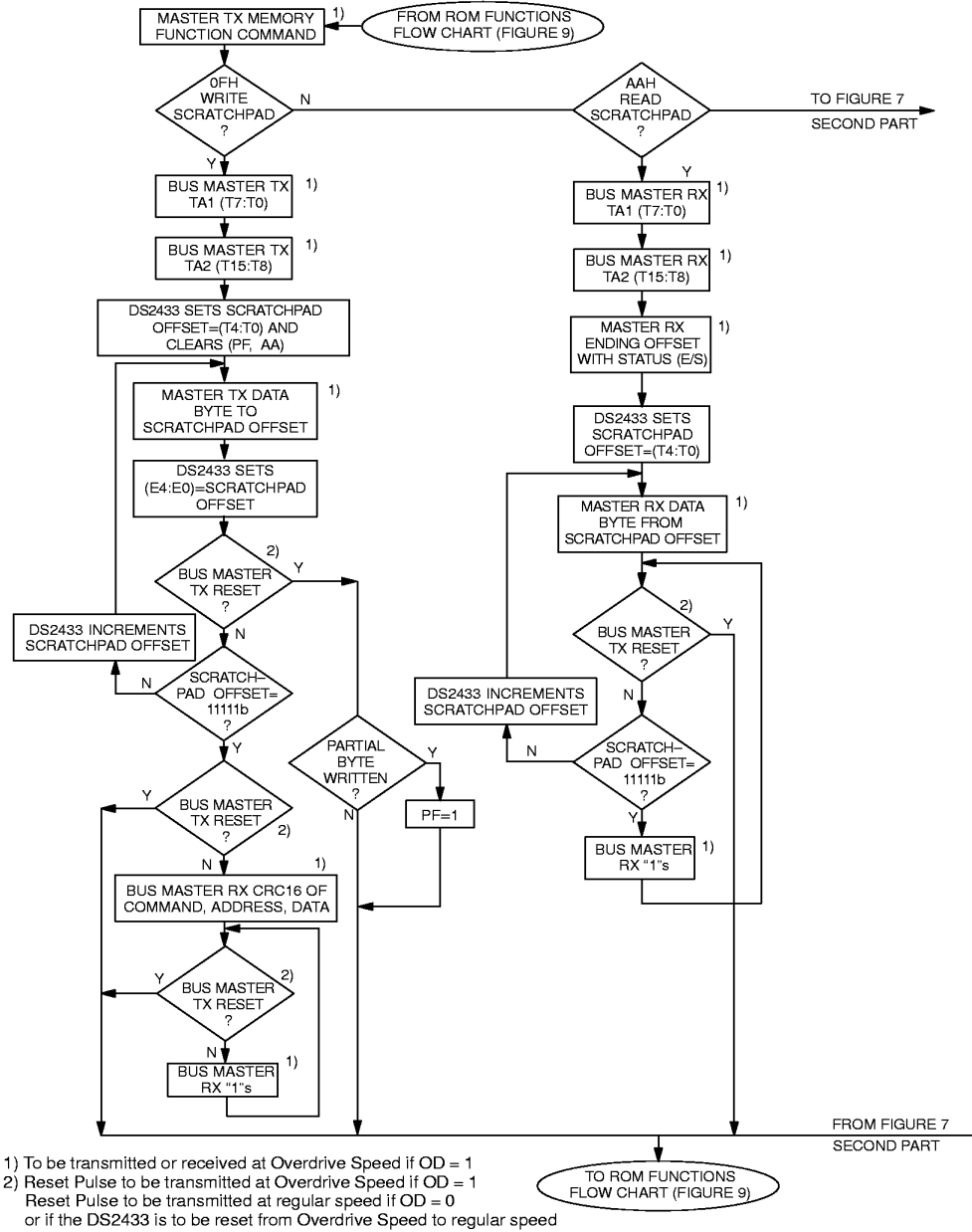
MEMORY FUNCTION FLOW CHART Figure 7
