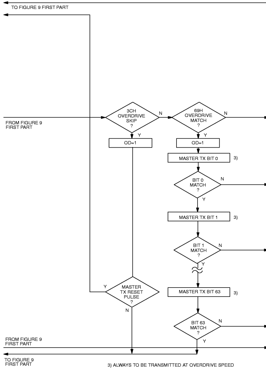
ROM FUNCTIONS FLOW CHART Figure 9 (continued)
