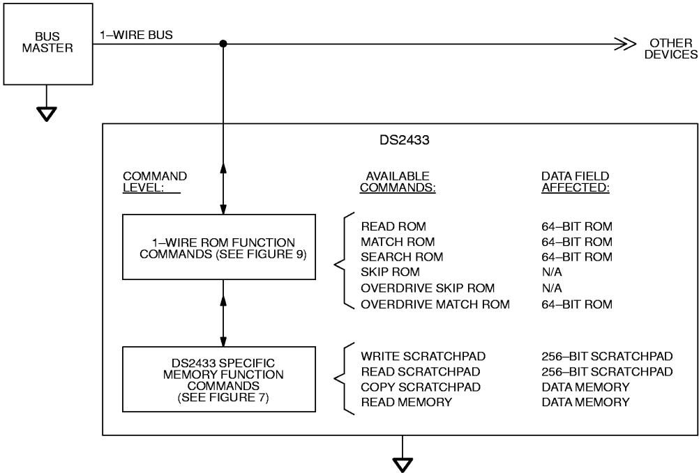
HIERARCHCAL STRUCTURE FOR 1-WIRE PROTOCOL Figure 2
