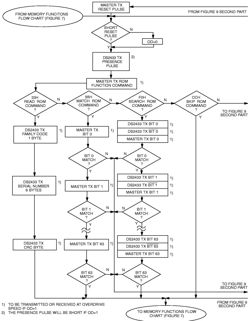
ROM FUNCTIONS FLOW CHART Figure 9 (First Part)
