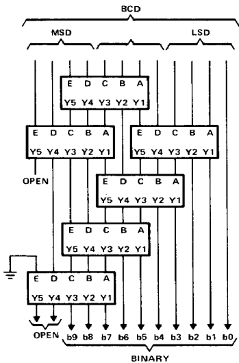
FIGURE 3—BCD-TO-BINARY CONVERTER FOR THREE BCD DECADES
