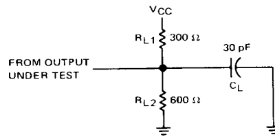
LOAD CIRCUIT FIGURE 1
