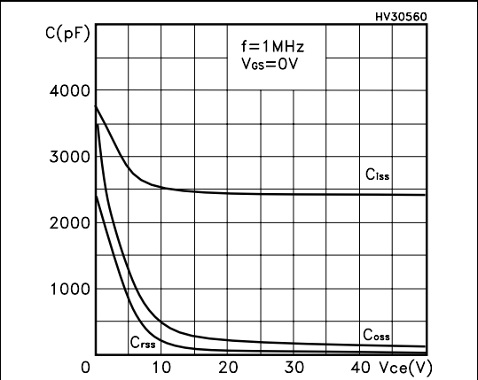
Figure 7. Capacitance variations
