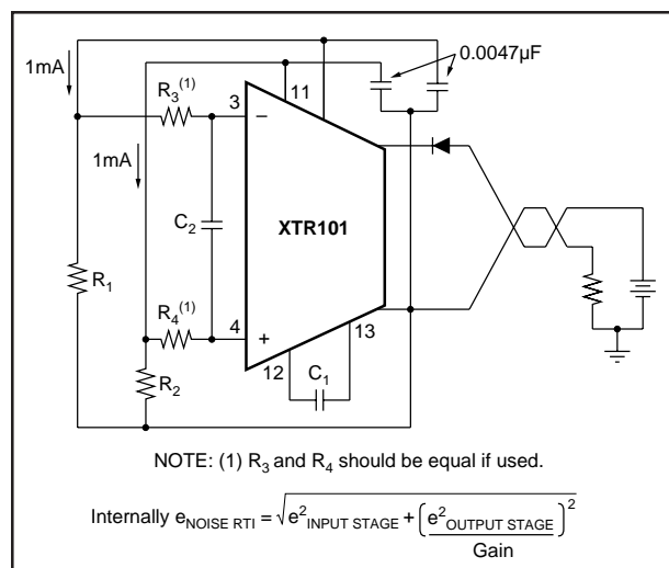
FIGURE 12. Optional Filtering.
