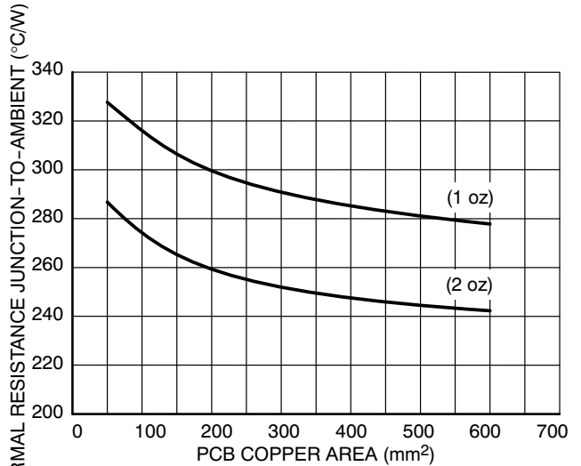
Figure 26. R thJA vs. PCB Copper Area
