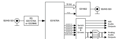
Application: Multi-format Audio De-embedder Module
