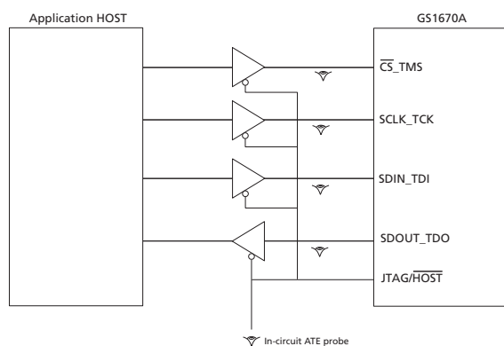
Figure 4-44: In-Circuit JTAG
