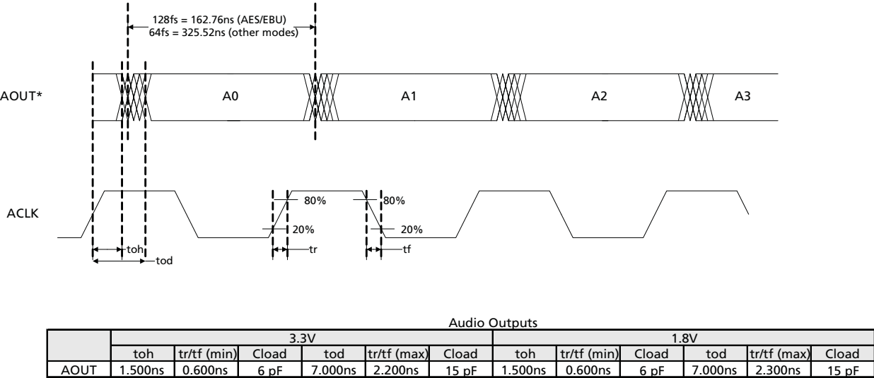
Figure 4-26: ACLK to Data Signal Output Timing
