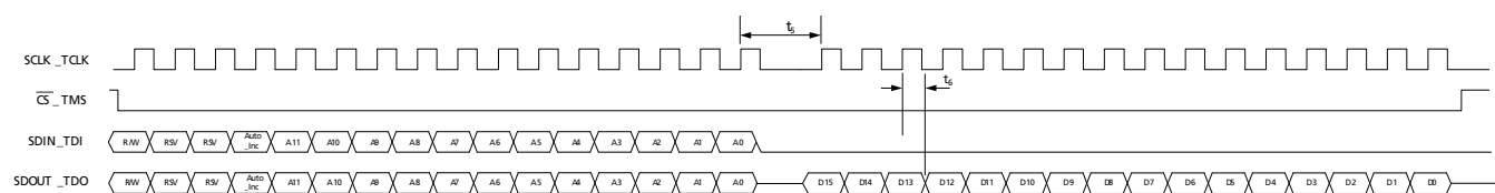
Figure 4-42: Read Mode
