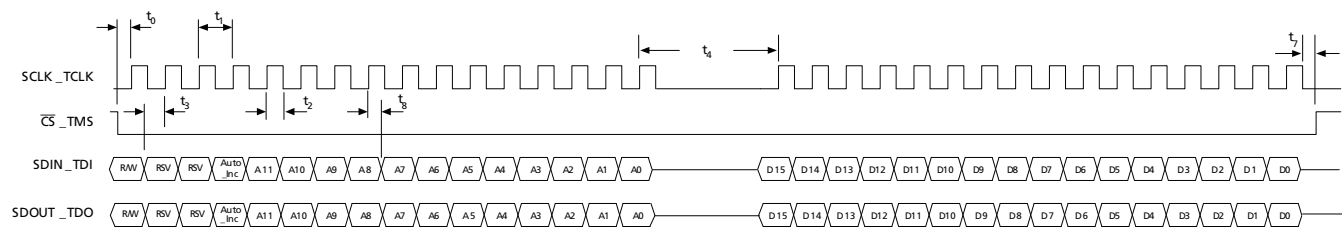
Figure 4-41: Write Mode
