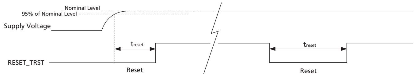
Figure 4-46: Reset Pulse
