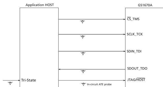
Figure 4-45: System JTAG
