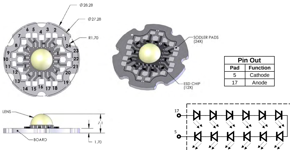
Figure 11: Standard MCPCB outline dimensions (mm).
