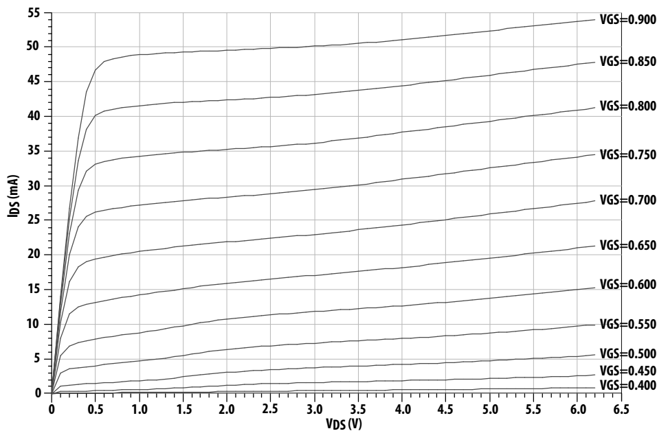
Figure 1. Typical I-V Curves. (VGS=0.05 V per step)
