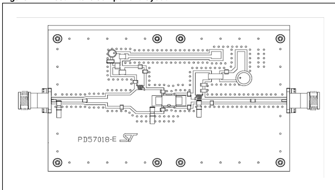
Figure 24. Test fixture component layout
