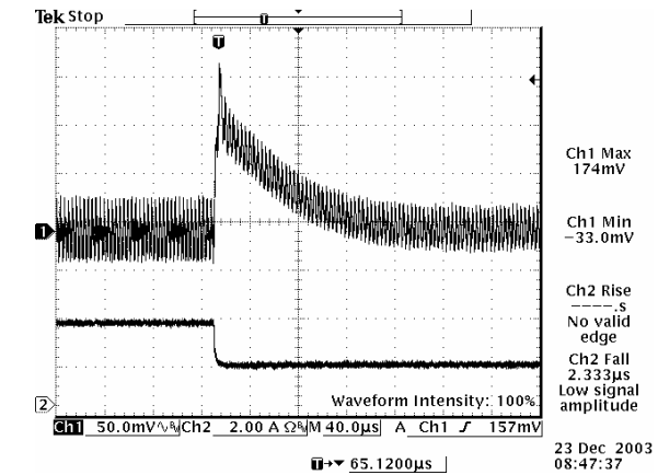
Transients 100% to 50% load 5 Vdc output
