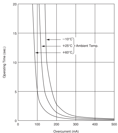
PRG21BB150MB1RK
