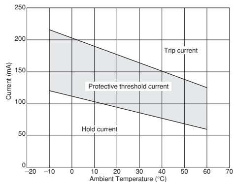
PRG15BC4R7MM1RC
