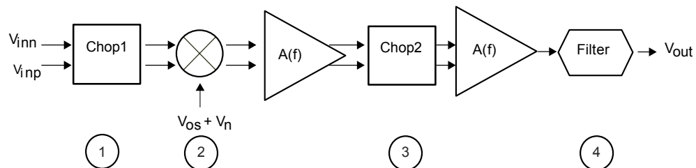
Figure 49. Block diagram in the frequency domain
