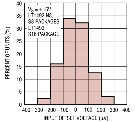
Distribution of Input Offset Voltage
