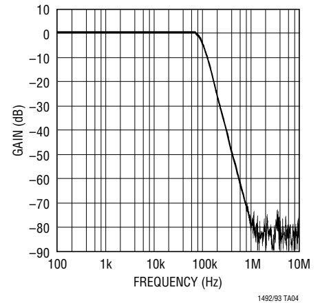
Frequency Response
