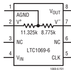
Figure 1. Internal Biasing of the Analog Ground (Pin 1)
