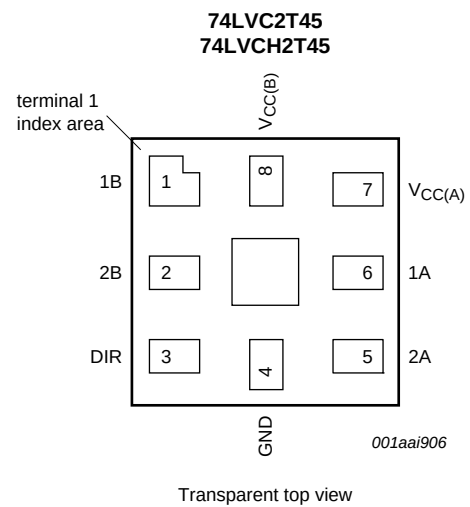
Fig 6. Pin configuration SOT902-2
