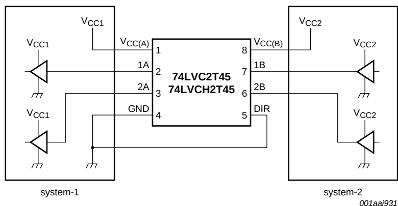
Fig 16. Unidirectional logic level-shifting application
