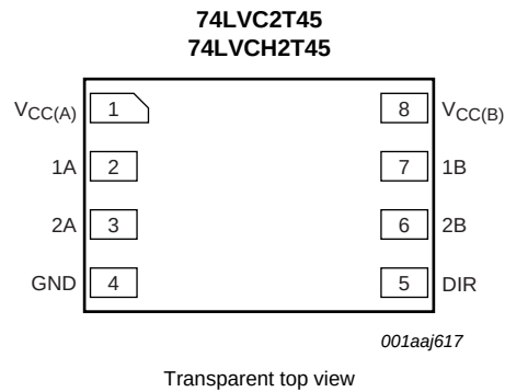
Fig 5. Pin configuration SOT996-2
