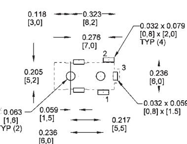
PC BOARD LAYOUT COMPONENT SIDE
