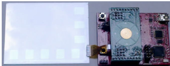
Figure 1. Capacitive Sense BoosterPack With LaunchPad
