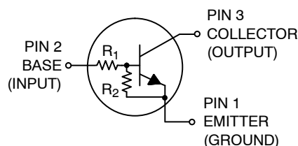
SC-59 CASE 318D STYLE 1
