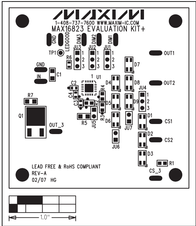
Figure 2. MAX16823 EV Kit Component Placement Guide—Components Side
