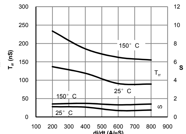
Fig 24: Diode Reverse Recovery Time and Softness Factor vs. di/dt ( V_{GE}=15V, V_{CE}=400V, I_F=30A )
