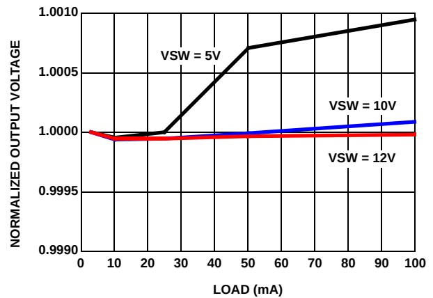
FIGURE 4. VSW REGULATION vs LOAD @ VPWR = 18V, AUXIN = 15V, +25°C
