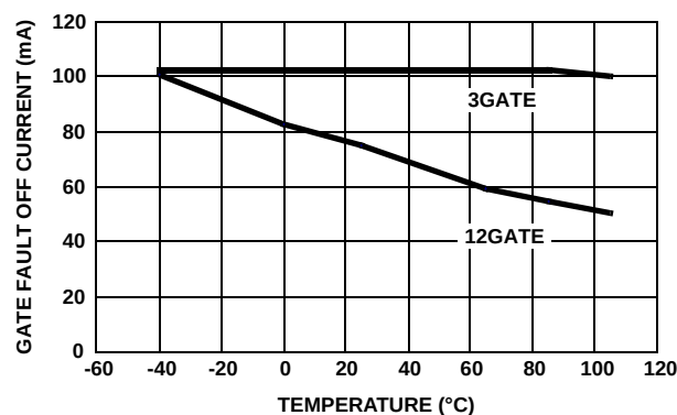
FIGURE 14. GATE FAULT OFF CURRENT (ABS) vs TEMPERATURE
