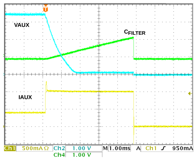
FIGURE 26. VAUX WOC REGULATION AND SHUT-DOWN
