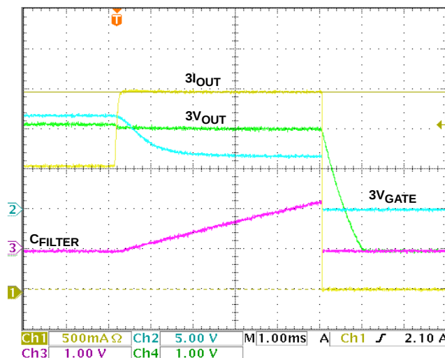
FIGURE 29. 3VMAIN CR AND SHUT-DOWN
