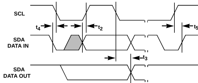
FIGURE 31. SMBUS TIMING
