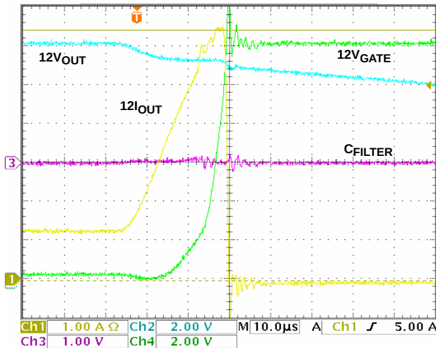
FIGURE 23. 12VMAIN WOC SHUT-DOWN
