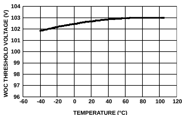
FIGURE 1. FAST TRIP THRESHOLD VOLTAGE vs TEMPERATURE
