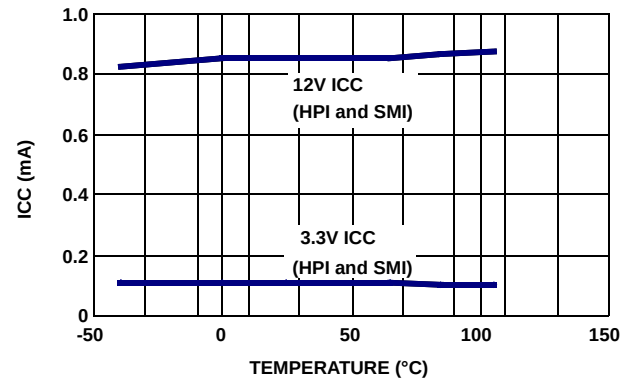
FIGURE 4. ICC CURRENT vs TEMPERATURE
