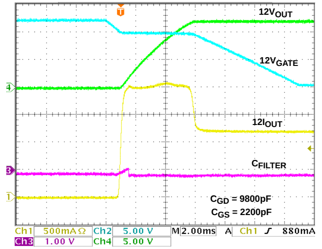
FIGURE 22. 12VMAIN START-UP R_{LOAD} = 10\Omega , C_{LOAD} = 470\mu F
