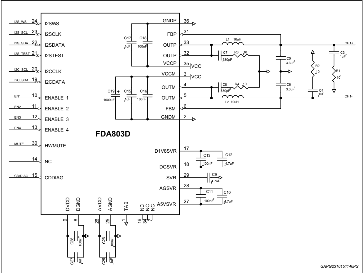
Figure 3. Application diagram
