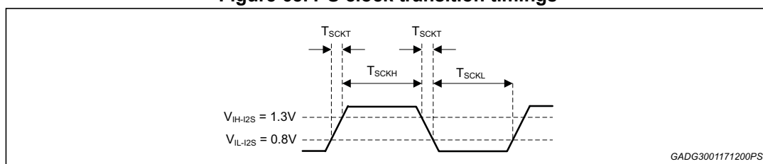
Figure 68. I 2 S clock transition timings
