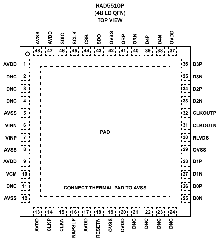
FIGURE 1. PIN CONFIGURATION
