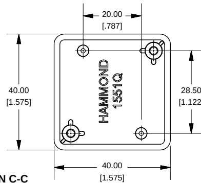
SECTION C-C Boss Heights
