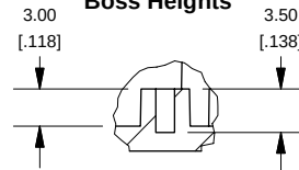
SECTION C-C Boss Heights
