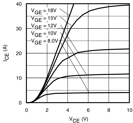
Fig. 7 - Typ. IGBT Output Characteristics T_J = 175^\circ\text{C} ; t_p = 80\mu\text{s}
