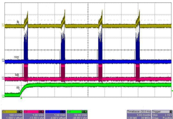
Figure 18. Soft-Start Waveforms
