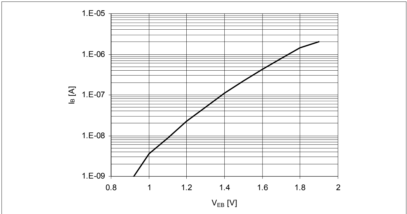
Figure 5-6 Base Current vs. Base Emitter Reverse Voltage I_B = f(V_{EB}) , V_{CE} = 2 V
