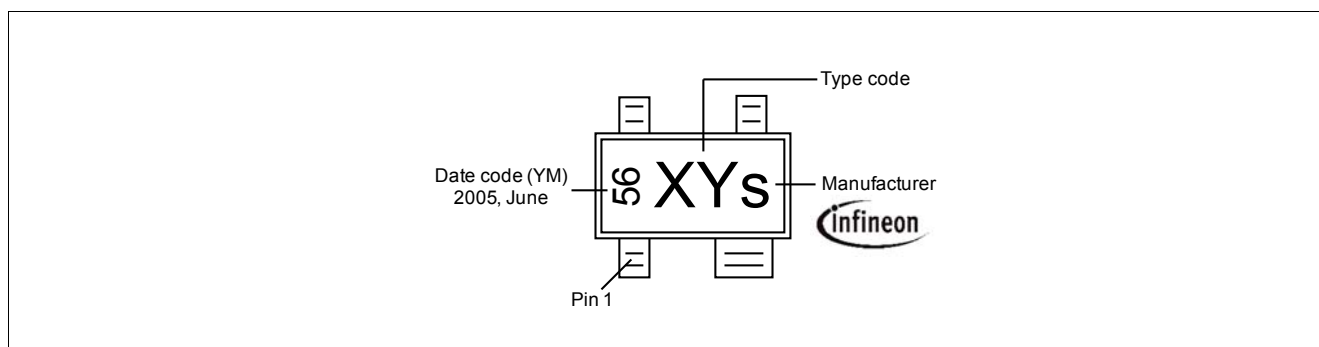
Figure 7-3 Marking Example (Marking BFP650: R5s)
