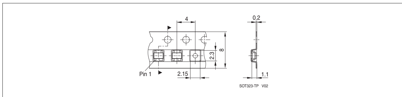
Figure 7-4 Tape dimensions
