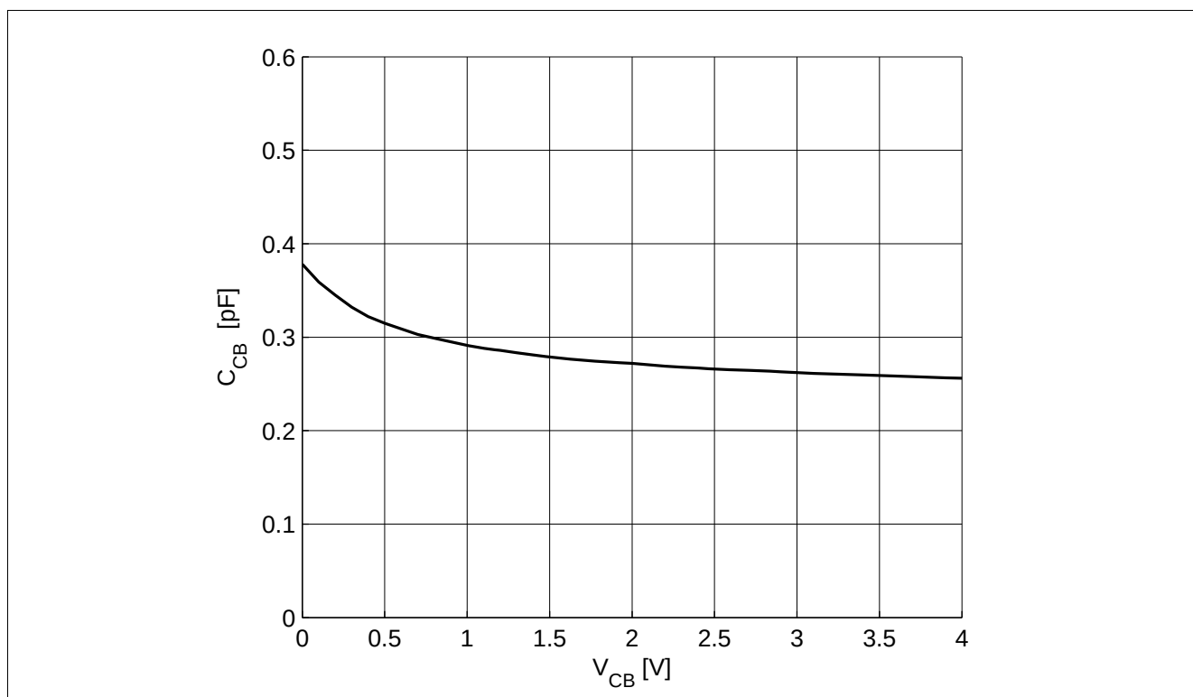
Figure 5-9 Collector Base Capacitance C_{CCB} = f(V_{CB}) , f = 1 MHz
