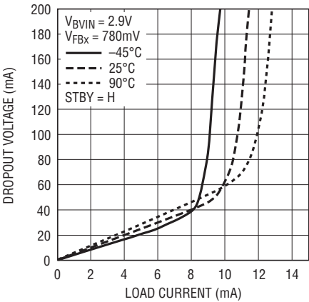
Step-Down Switching Regulator Dropout Voltage in Standby Mode vs Load Current
