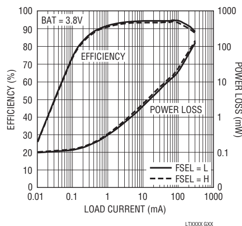
Figure 5. 3.3V Output Efficiency and Power Loss vs Load Current
