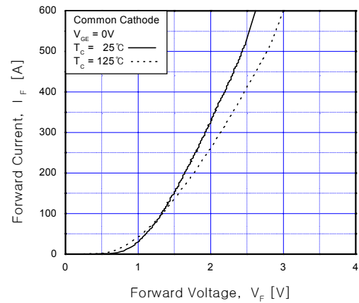
Fig 12. Forward Characteristics(diode)
