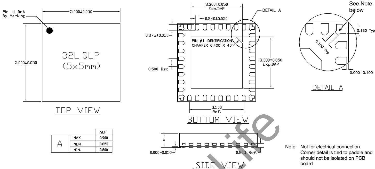
Figure 14. Package Drawing
