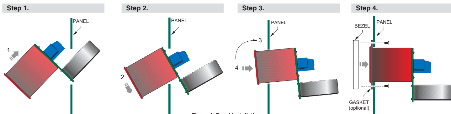
Figure 2. Panel Installation
