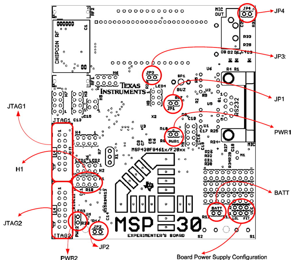
Figure 6. Jumper Locations
