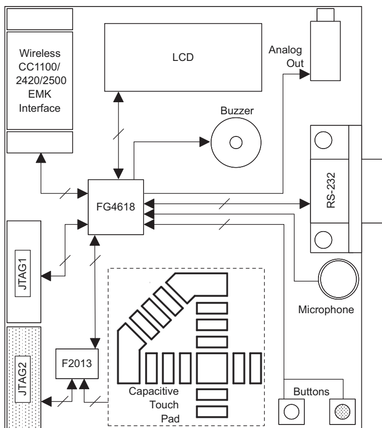
Figure 2. MSP-EXP430FG4618 Block Diagram
