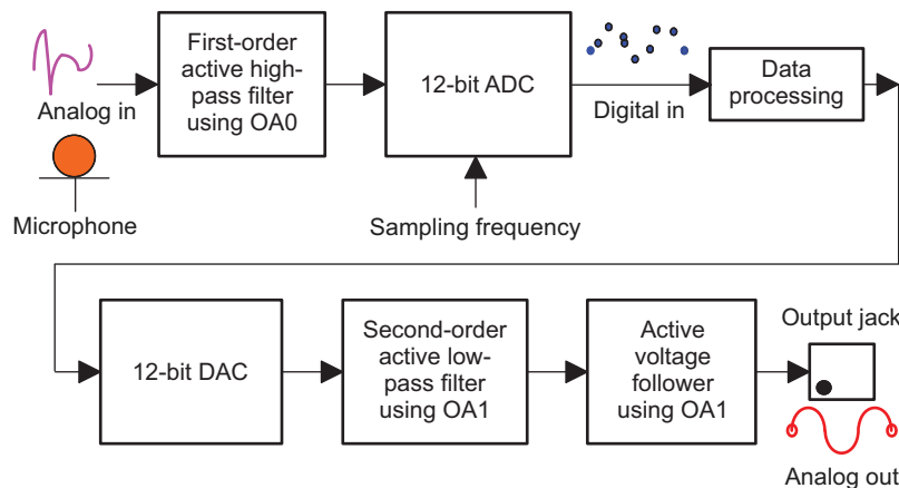
Figure 4. Analog Signal Chain of MSP430 MCU
