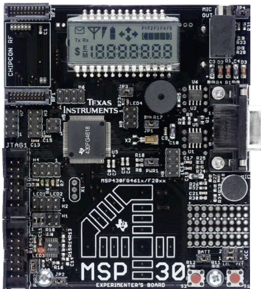
Figure 1. MSP430FG4618/F2013 Experimenter Board
