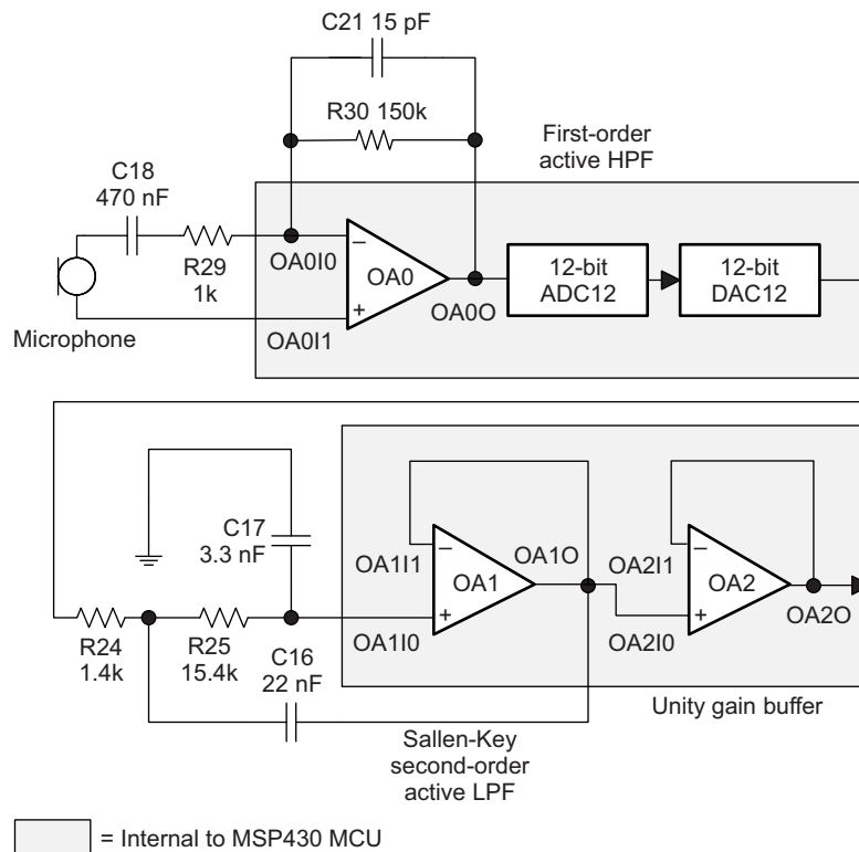
Figure 5. Active Analog Filter
