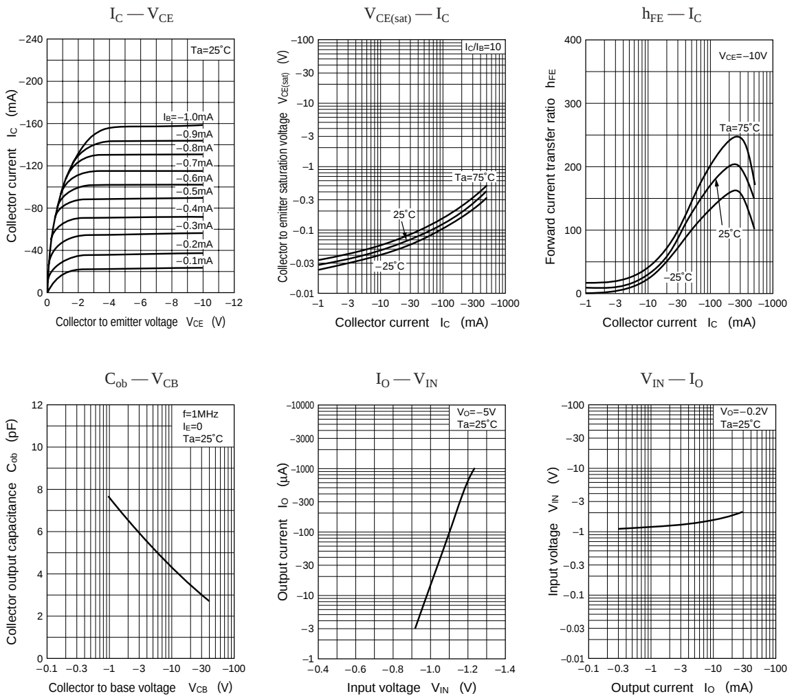
Characteristics charts of UN4122
