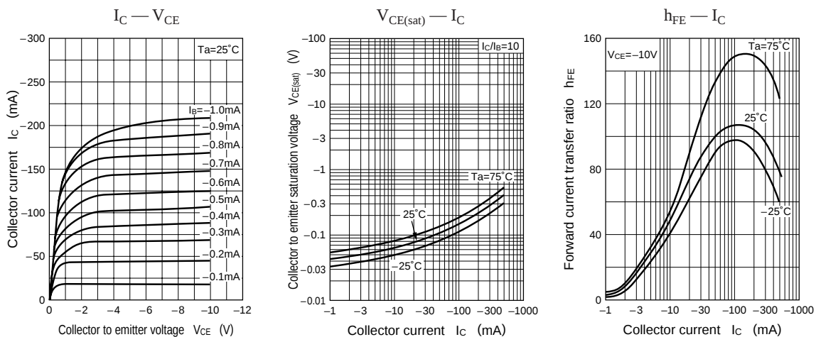
Characteristics charts of UN4122
