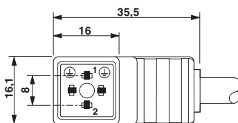
Valve connector, type C
